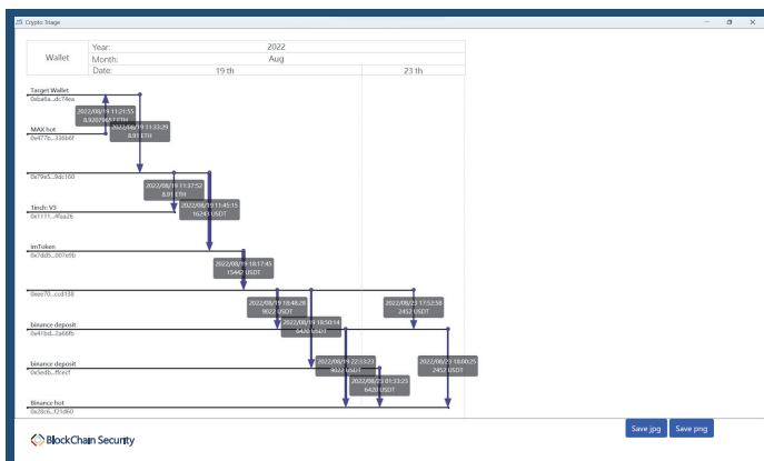
Timeline mode
