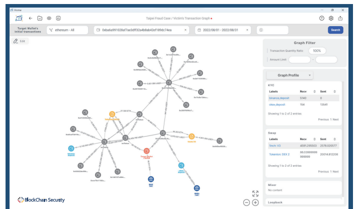
Wallet mode
